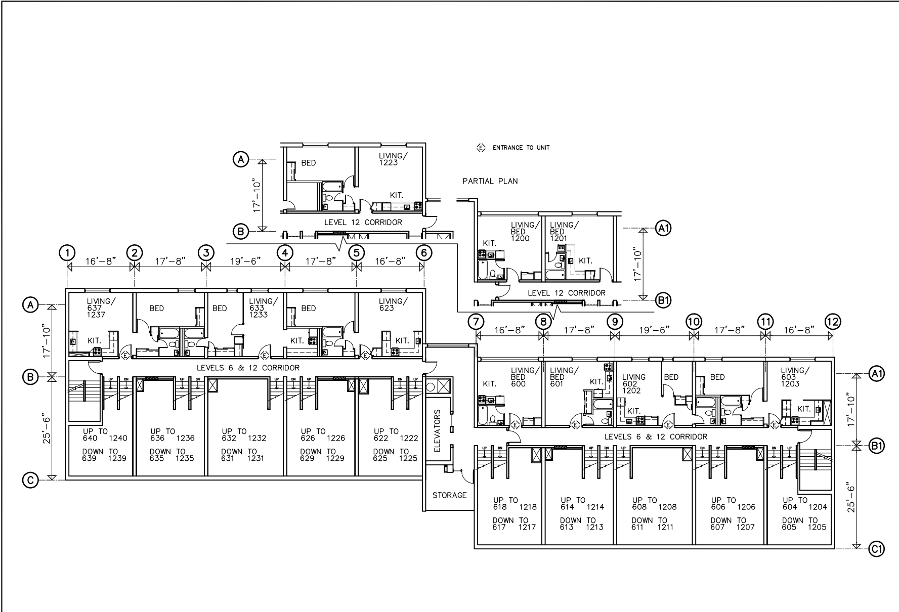
LEVELS 6 & 12
